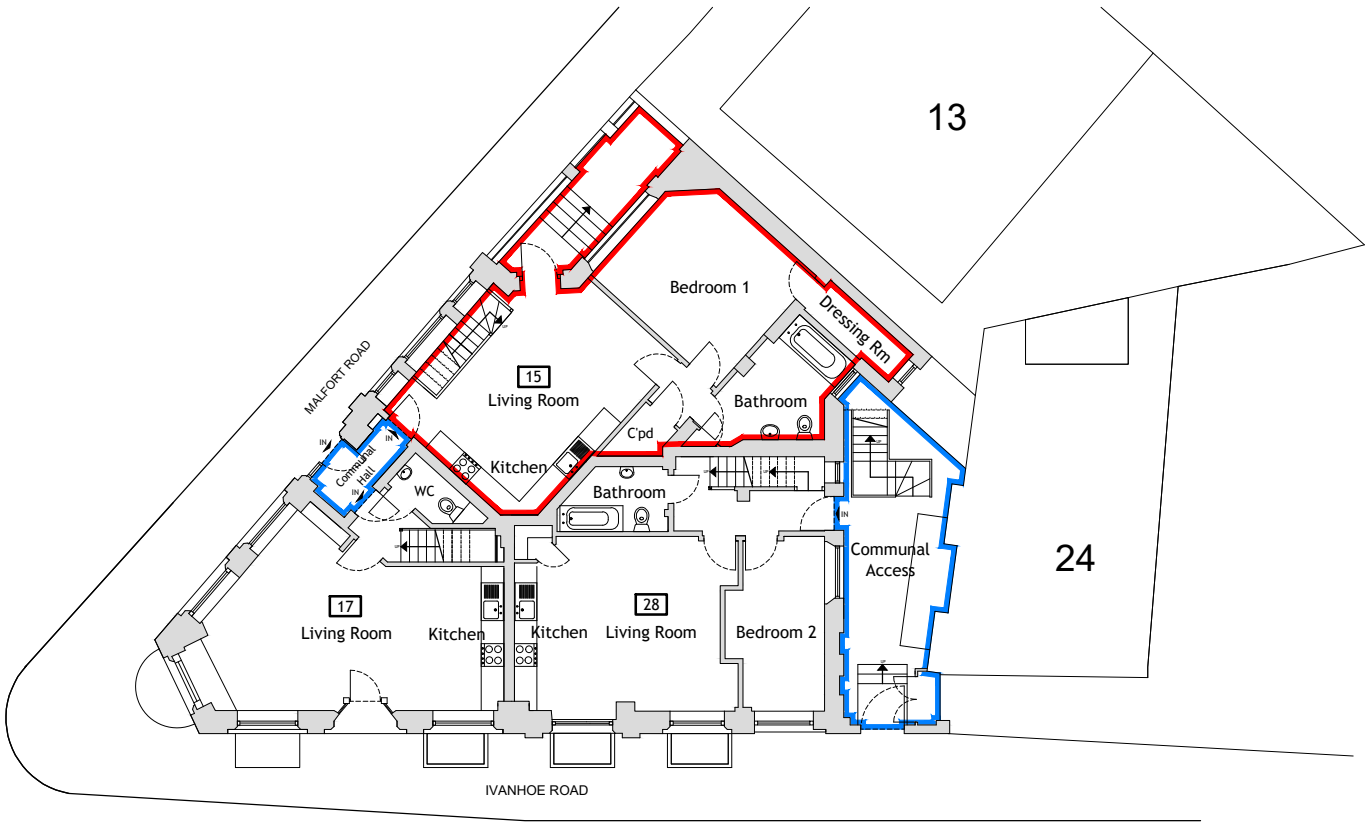
+00 Ground Floor Plan
