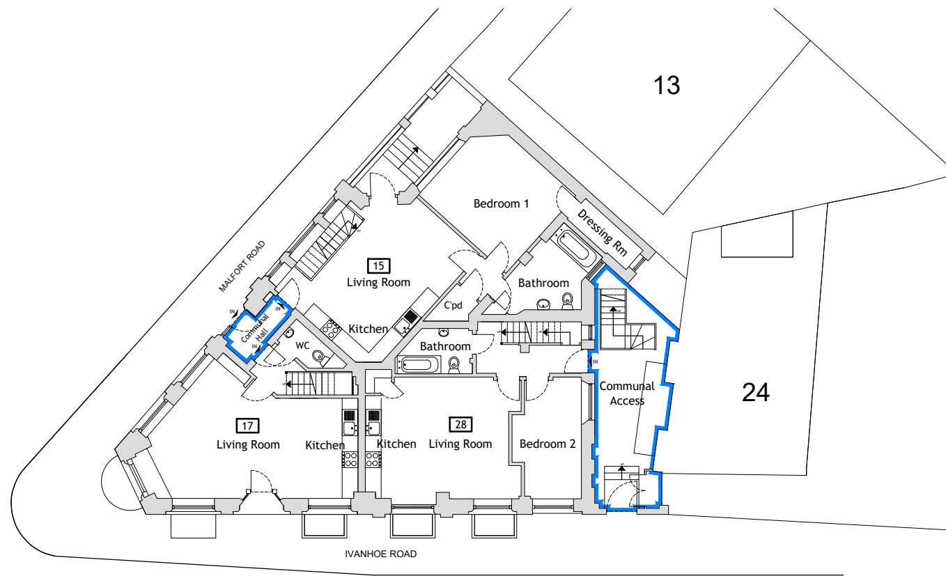
+00 Ground Floor Plan
