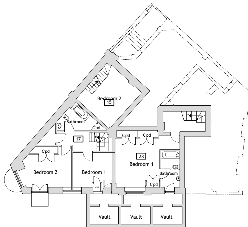
-01 Lower Ground Plan
