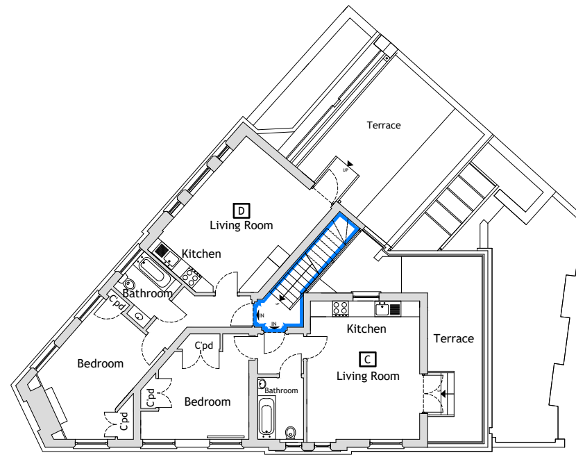
+02 Second Floor Plan
